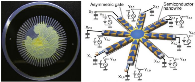
(Left) An amoeboid organism, like the slime mold Physarum polycephalum shown here on a gold-coated chip in an agar plate, provides a model of the computing principles of biological systems. (Right) Researchers designed a network of electrical Brownian ratchets to implement an amoeba-inspired computing system. Credit: M. Aono, et al. ©2015 IOP Publishing
